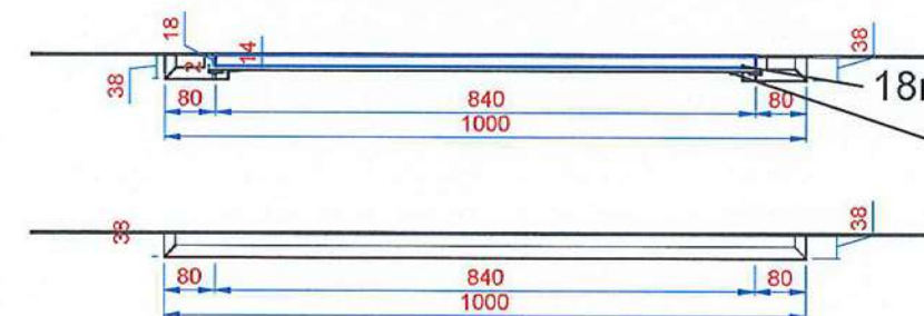
WOOD PANEL IN ROOMS With Art Work
