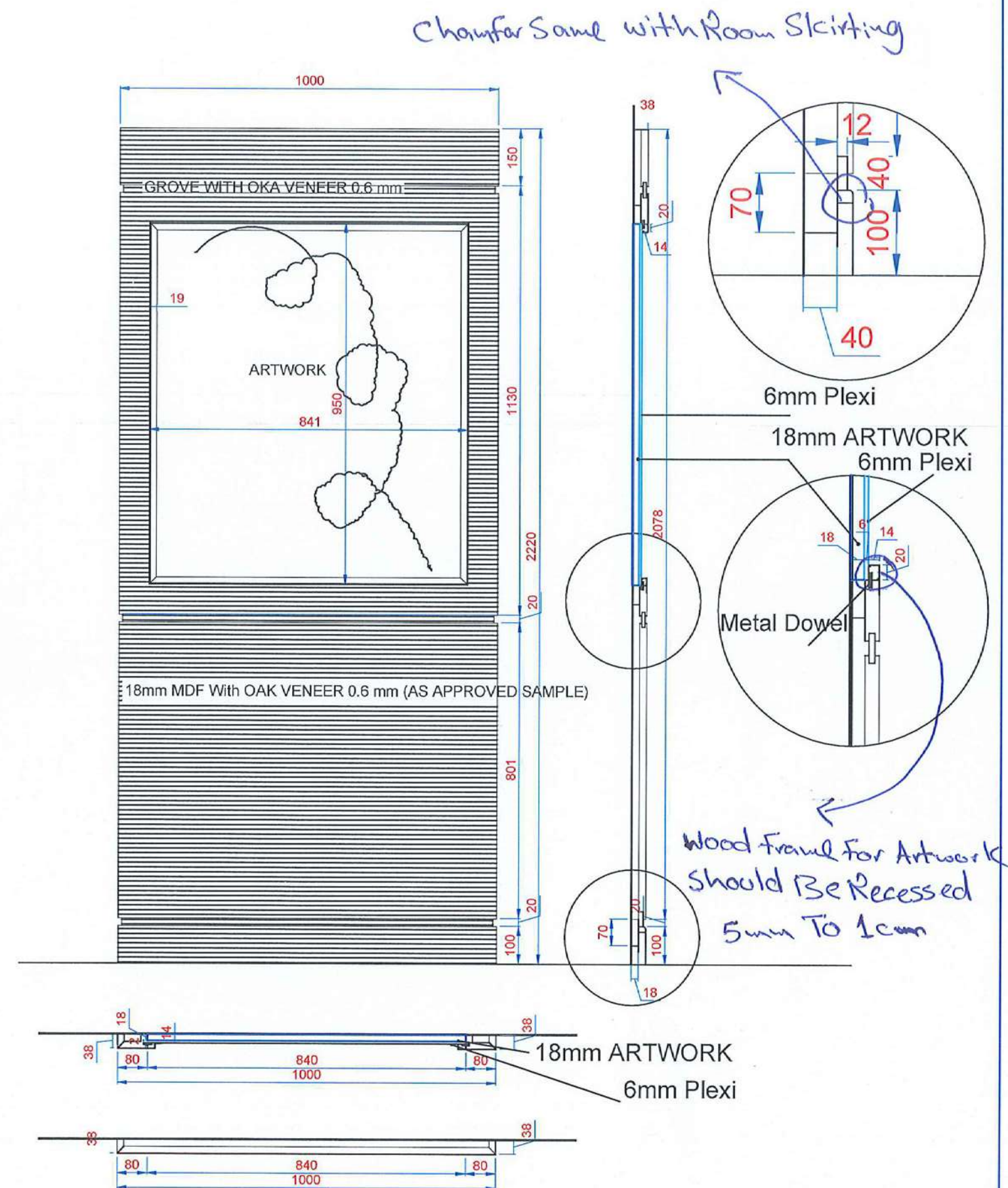
WOOD PANEL IN ROOMS With Art Work
