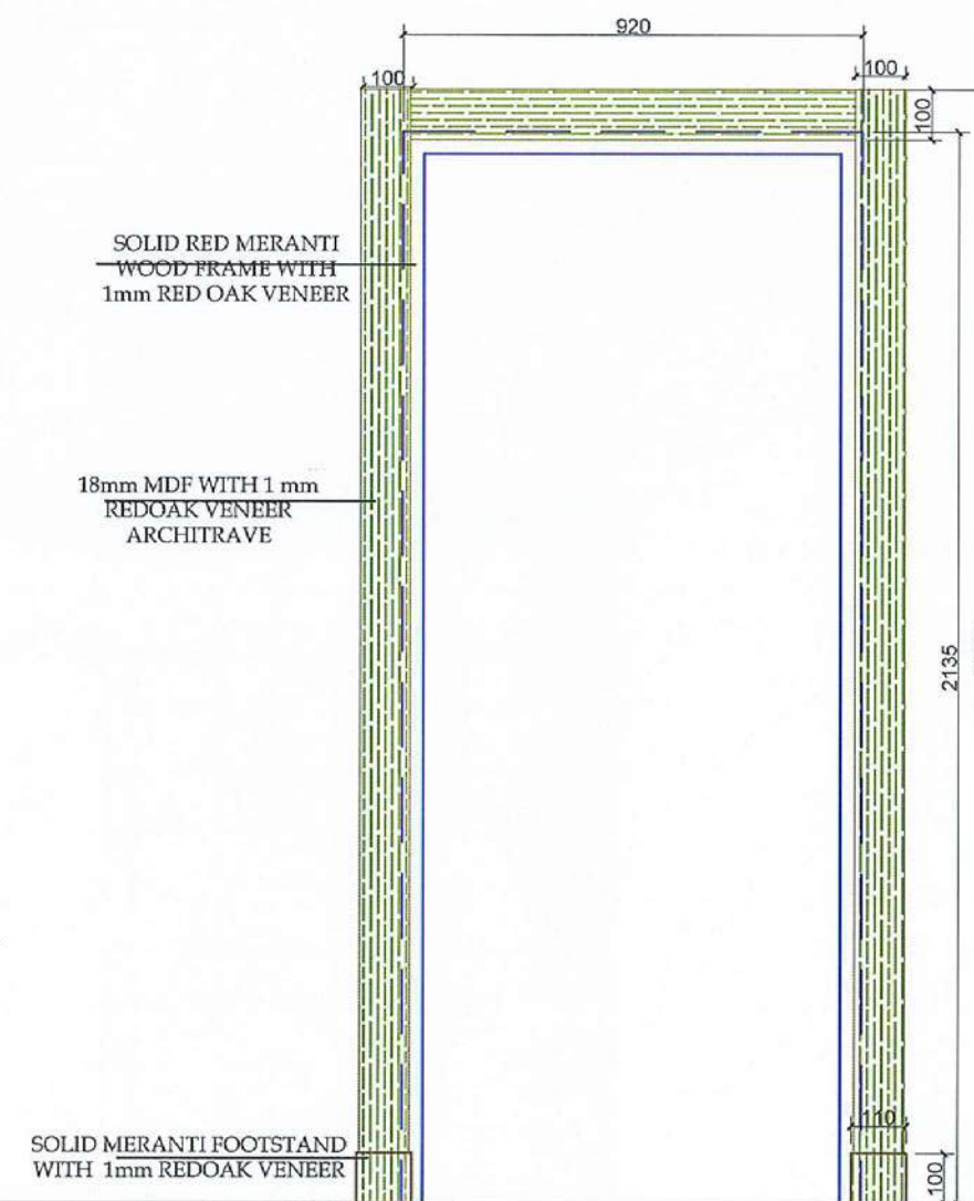
FRAME DETAIL FRONT ELEVATION SCALE: 1:5
