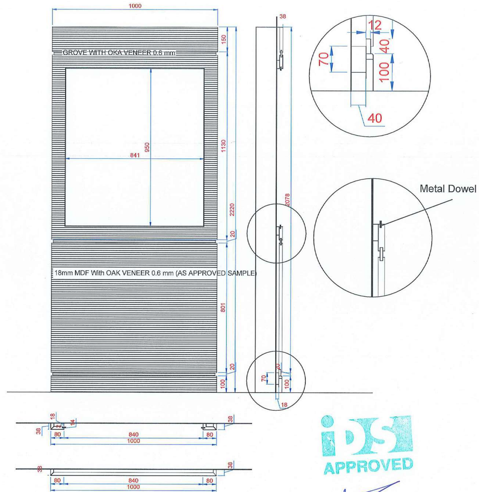
WOOD PANEL IN ROOMS Without Art Work
