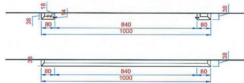
WOOD PANEL IN ROOMS Without Art Work
